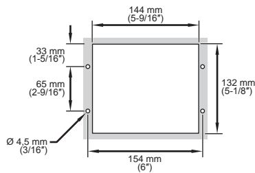
RCTHW-1B Control Box Cutout Dimensions
